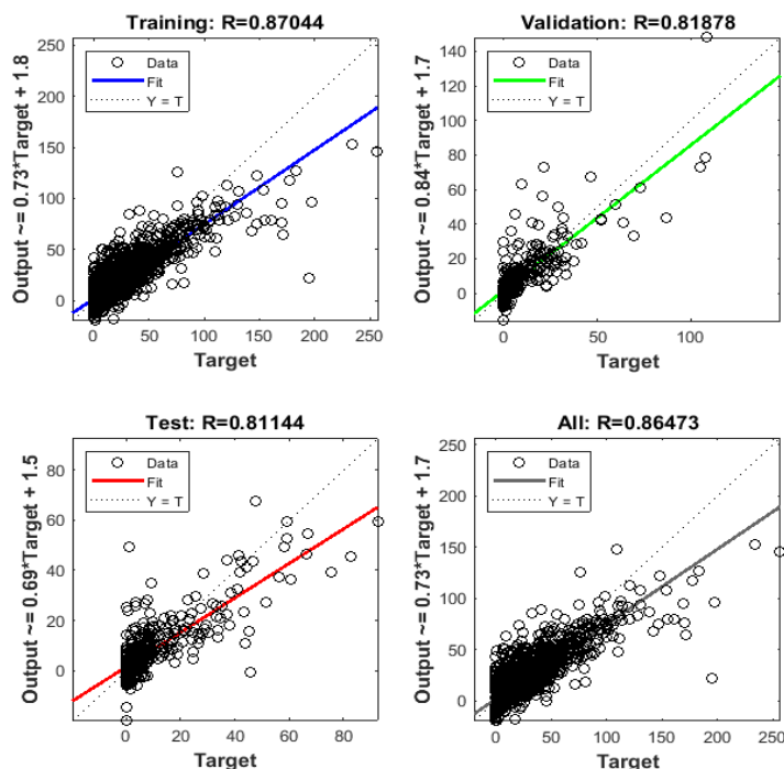
Fig-4: Regression plot of Levenberg Marquadt Predictive Algorithm
