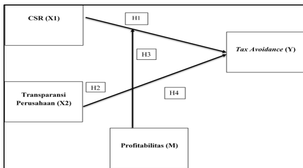
Picture-1: Framework
